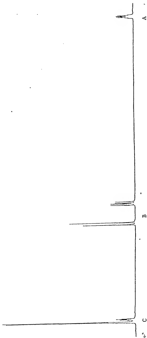
Figure 81 - ^{19}\text{F} NMR of \text{CF}_2\text{C}(\text{F})\text{C}(\text{F})\text{CH}_2\text{CH}=\text{CF}_2 C A B
